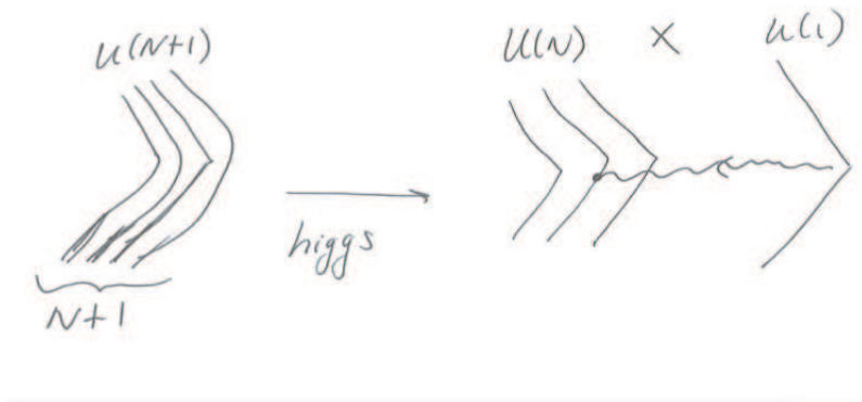
Figure 1: One of the D3 branes is separated from the other N , thus breaking the U(N + 1) down to U(N) \times U(1) .
