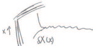
Figure 3: The string pulls on the stack of D3 branes, so it couples to the adjoint scalars.
