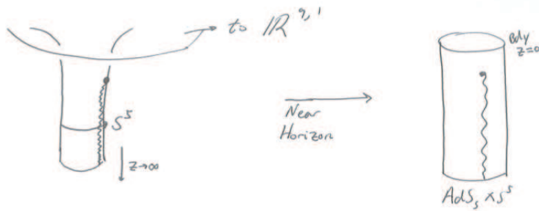
Figure 2: The string stretches into the throat from the probe D3 brane at z_w .
