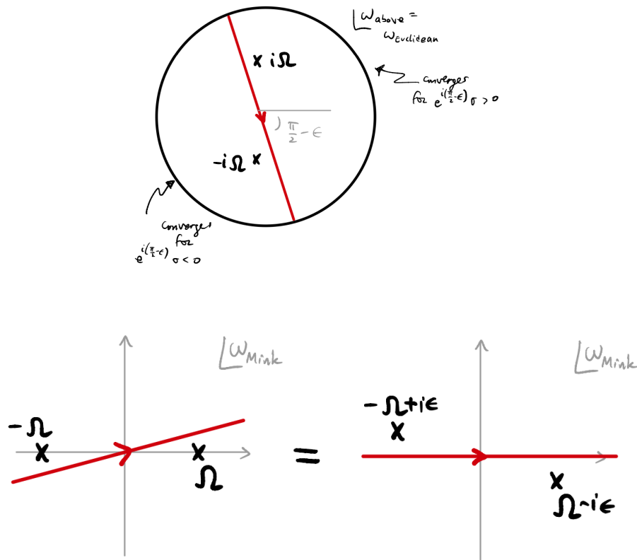
Figure 2: The Feynman contour in the \omega_{\text{Mink}} complex plane.
