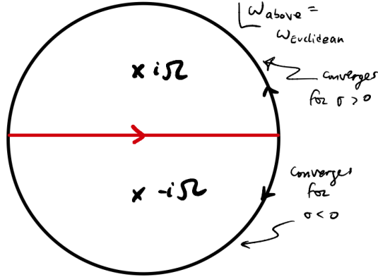
Figure 1: Poles of the integrand of the \omega integral in (2.13).
