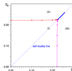
[from Tupitsyn-Kitaev-Prokof'ev-Stamp ]
