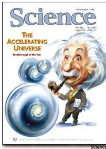
Fig. 4.— Science Magazine named the discovery of the Accelerating Universe the top science breakthrough of 1998. Thus we see why Einstein's caricature above is pleasantly surprised at the possibility that \Lambda might not have been a blunder after all. The sheer excitement of this result was undoubtedly one of the reasons I joined the Filippenko group in early 1999.
