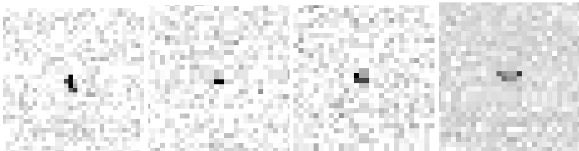
Fig. 10.— Here are a few examples of what individual cosmic rays look like on the CCD when this same image is magnified. Cosmic rays generally take up only a few pixels and sometimes just a single pixel. You are probably already familiar with this from the supernova search, where cosmic rays often appear, for a moment, to be good supernova candidates until you see that their profile is more like a spike or delta function than a starlike Gaussian.
