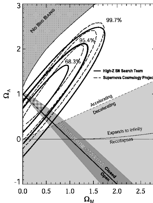
Fig. 6.— Summary of the HZT-SCP Cosmological Parameter Measurements, graphed in the \Omega_M vs. \Omega_\lambda plane. Galaxy cluster measurements also indicate independently that \Omega_M \approx 0.3 , representing another vertical strip that happens to also intersect the combined Supernova and CMB data. Thus we see a convergence in the data from the HZT, SCP, BOOMERanG and MAXIMA collaborations at around \Omega_M \approx 0.3 and \Omega_\lambda \approx 0.7 . Results from DASI are not shown. This convergence very strongly suggests that the universe is accelerating due to a nonzero cosmological constant \Lambda .
