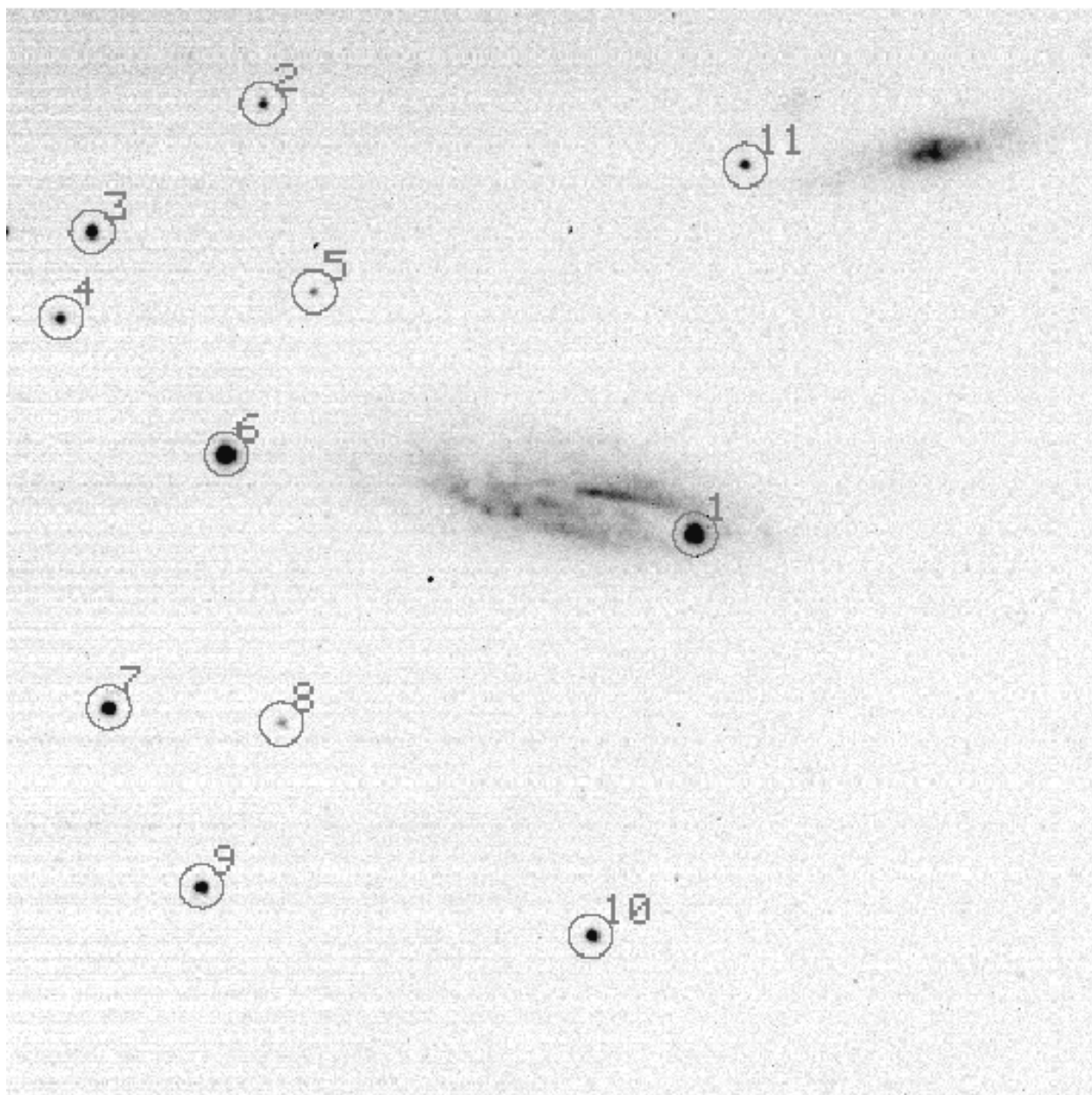
Fig. 7.— An example finding chart for supernova 1998dh. In the chosen image, which happened to be taken on 8/2/98, the supernova is numbered “1” and the secondary standard stars in the field are numbered “2,3,4...” in an arbitrary order which you choose at the beginning, but which you must keep consistently throughout the process. The finding chart is a useful reference to keep at hand while doing photometry.
