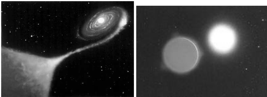
Fig. 5.— Artist’s conceptions of the single degenerate and double degenerate scenario for Type Ia supernovae. Artist Credit: Dana Berry and Dan Durda.
