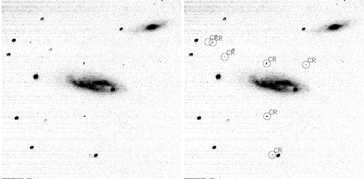
Fig. 9.— Here is an example of what cosmic rays look like in a B band image of supernova 1998dh taken on 8/20/98. As usual, there are number of cosmic rays in the image, which are highlighted with circles in the second frame.
