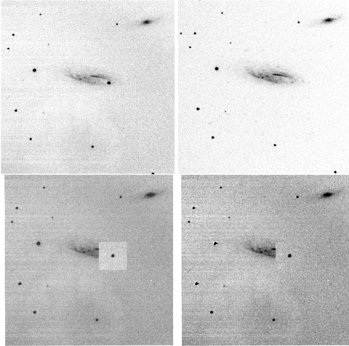
Fig. 14.— An example image from supernova 1998dh taken on 8/12/98 is shown going through the galaxy subtraction process with both pipelines, each using a galaxy template image taken on 7/19/2001. Upper left: The original supernova image. Upper right: The galaxy template where the supernova is not in the image. Lower left: The galaxy subtracted image of the supernova obtained using the High-Z pipeline. Lower right: The galaxy subtracted image of the supernova obtained using Weidong's pipeline. Notice the easily apparent search boxes surrounding the supernova with galaxy light removed. Notice also that all images are 500 x 500 pixel squares of the same size and that both the galaxy subtracted images appear to have an L-shaped section missing on their lower left (which just appears white). This occurs because the galaxy subtraction program fsn2 registers the images to the same coordinates as the galaxy template, which had a slightly shifted field of view. Note that if a different template was used, the shift to register the images might be different and the search boxes might appear at different [x_{left}:x_{right}, y_{bottom}:y_{top}] coordinates, for example [266:346, 216:296] , rather than [287:367, 228:308] as in the above images.
