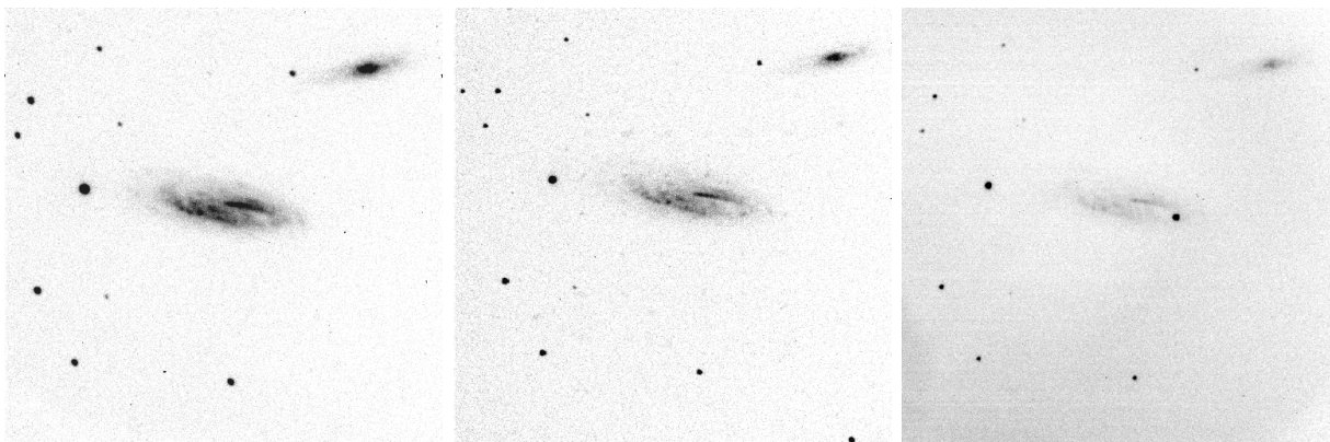
Fig. 13.— (Left and Middle): Two example galaxy template calibration images for supernova 1998dh, where the supernova is not apparent. Both images were taken well after the supernova has become too faint to see (left: 9/25/2000 and middle: 7/19/2001), and can thus be used for galaxy subtraction. The final image on the right, taken on 8/7/1998, shows the supernova, (in the lower right corner of the host galaxy) for comparison.
