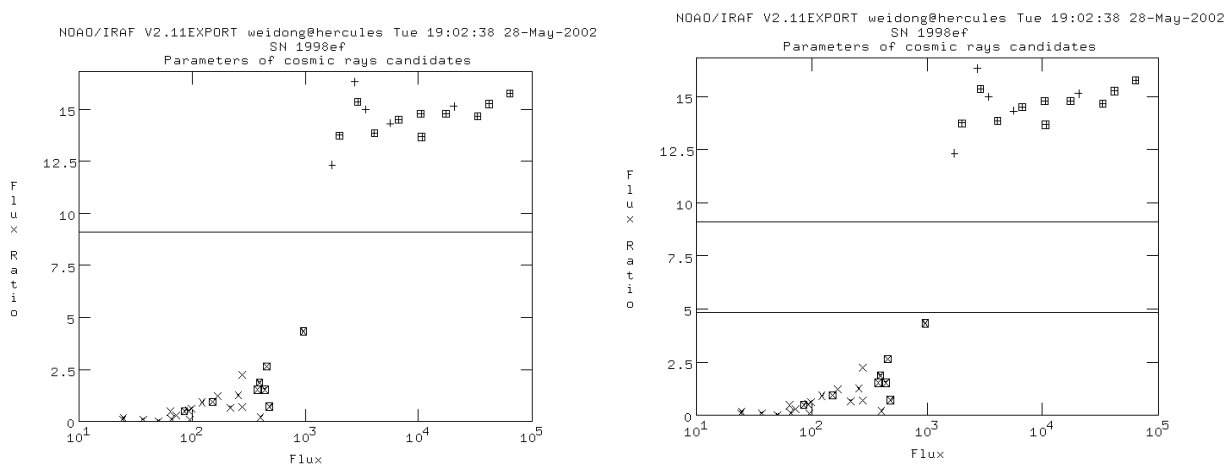
Fig. 11.— Plot of flux ratio vs. flux, for some objects in the image. Those detected as cosmic rays are marked with an “x”. Those detected as stars are marked with a “+”. Stars and cosmic rays that you identified by hand also have a box around the “+” or the “x”. In the second plot, we have adjusted the flux ratio to a lower value by hitting ‘t’ in the Tek window. Thus the second lower horizontal line.
