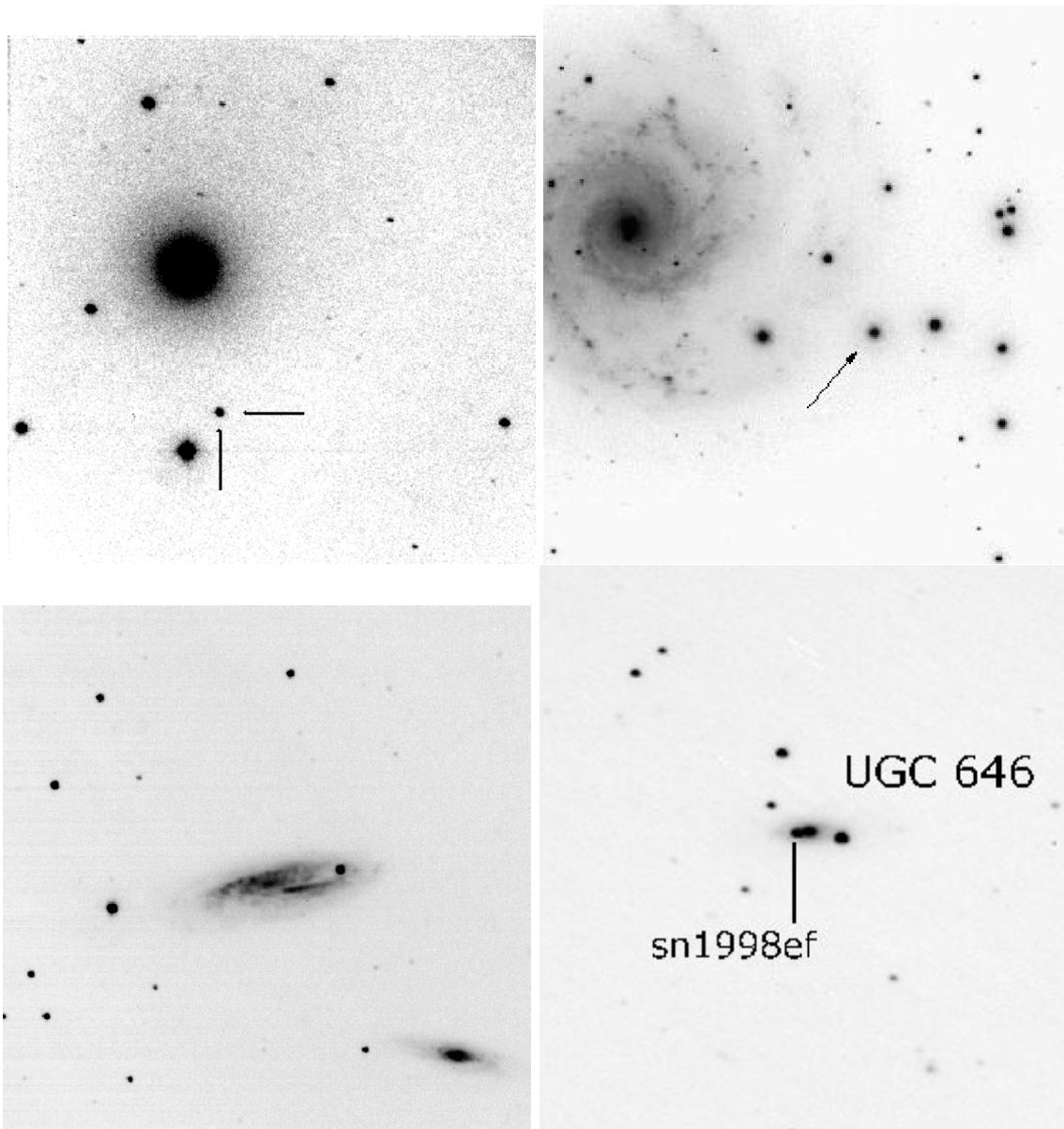
Fig. 12.— Some examples of supernovae that do or do not require galaxy subtraction. Row 1: (left to right) Supernovae 2000cx and 2002ap: They don't need galaxy subtraction because they occur far enough away from the nucleus of their host galaxy. Supernova 2000cx only required aperture photometry, while 2002ap also needed PSF photometry. Row 2: (left to right) Supernovae 1998dh (in upper right corner of host galaxy) and 1998ef: They do need galaxy subtraction because they occur close to the nucleus of their host galaxy. sn1998ef in particular is practically buried in the nucleus, ensuring that the galaxy light will be comparable to the supernova light in that region on the CCD image. Both these supernova required both aperture and PSF photometry.
