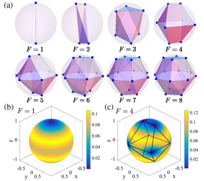
FIG. 3. Stable ground-state vortex configurations of dipolar Bose-Einstein condensate with g = 50 and different g_d . In (a), the data are obtained using g_d = 10 for F = 1-5 and g_d = 8 for F = 6-8 , respectively. The vortex cores are represented with blue dots on the spherical surface. Since the dipole-dipole interaction breaks the rotation symmetry, the pattern is only equivalent up to a global rotation around the z axis for each F . (b) and (c) show the selected density portraits for F = 1 and F = 4 , respectively. The vortices pattern is guided by lines and dot lines inside the sphere.
