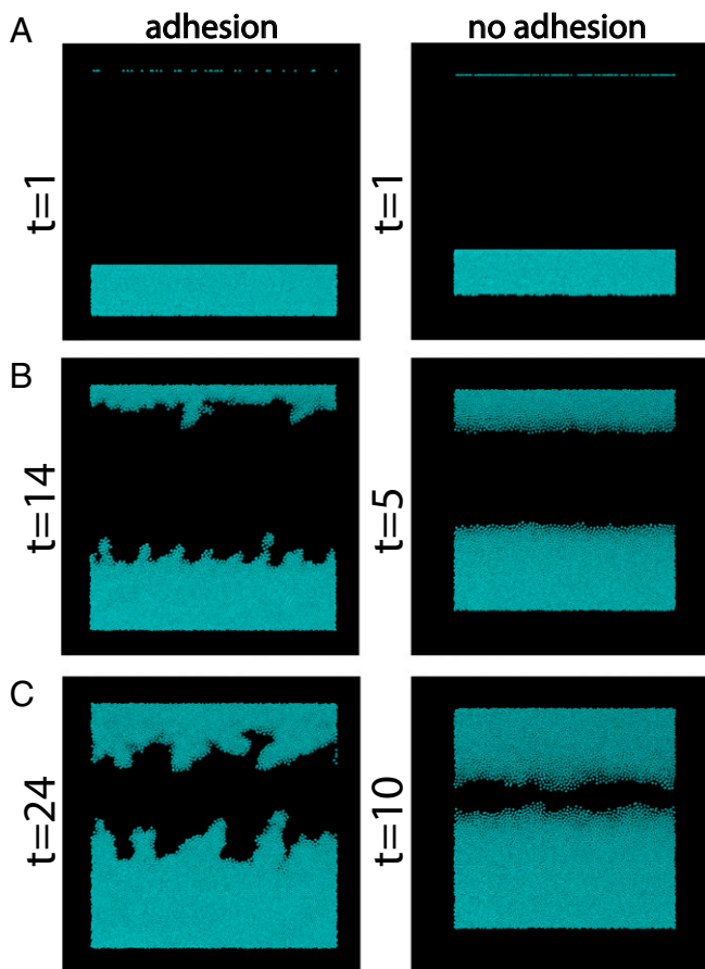
Fig. 6. Evolution of the edge of spreading tissues at different time points after removal of a hard wall in the y direction that was in place during initialization. Both tissues have identical parameters except that the adhesion force is set to zero in the tissue on the right-hand side, f_1 = 0. Whereas the adhesive tissue shows pronounced finger-like protrusions, the tissue without adhesion spreads much more uniformly, consistent with our analysis (Movies S7 and S8). The parameters deviating from the standard tissue are given by (k^\pm)^* = 0.1, k_{\text{mot}}^* = 0.025, m^* = 0.83, k_{\text{div}}^* = 0.5, and \xi_{\text{int}}^* = 0.2.
